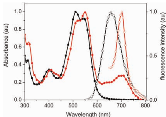
Figure 3. Normalized fluorescence (open symbol) and absorption (solid symbol) spectra of the thin solid films of Spiro-PDI 1 (black) and Spiro-PDI 2 (red).
