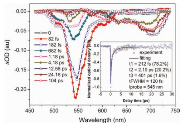
Figure 2. Transient absorption spectra of Spiro-PDI 2 in toluene after excitation at 530 nm with a 120 fs pulse of laser. The inset shows the dynamic decay of the bleaching at 545 nm and the fitting results.
