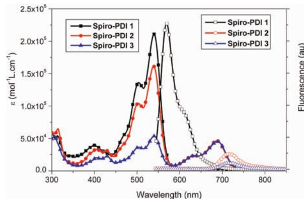
Figure 1. Absorption (solid symbol) and fluorescence (open symbol) spectra of Spiro-PDI 1 (black), Spiro-PDI 2 (red), and Spiro-PDI 3 (blue) in toluene.
