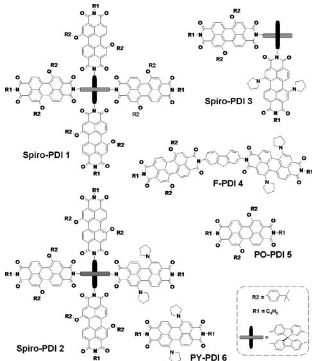
Scheme 1. Molecular Structures of the Compounds
